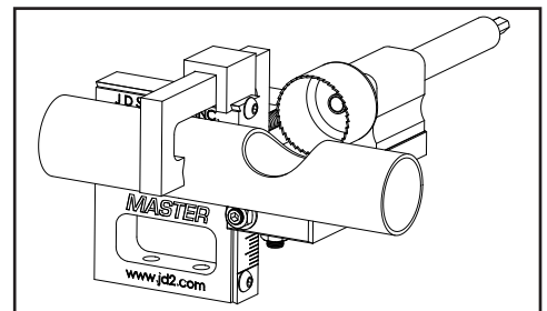
Offset Notches
