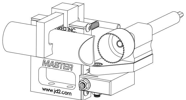
Figure 3 - Making a Straight Notch
